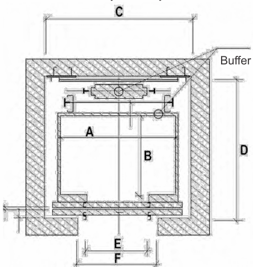
Hoistway Plan Layout
